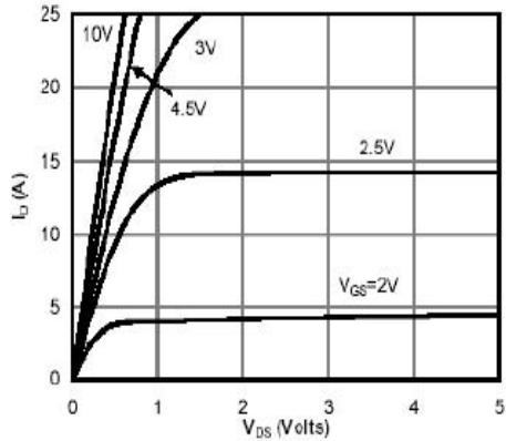
Fig 1: On-Region Characteristics
