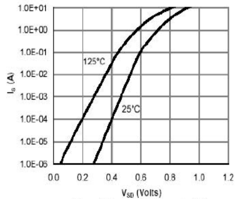
Figure 6: Body-Diode Characteristics
